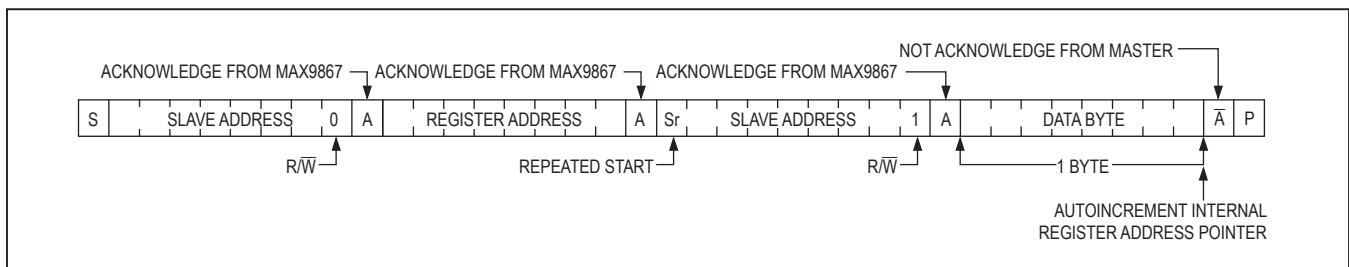
Figure 14. Reading 1 Byte of Data from the MAX9867
