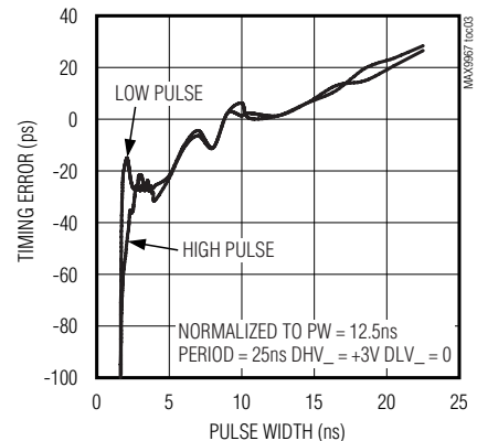
DRIVER TRAILING EDGE TIMING ERROR vs. PULSE WIDTH
