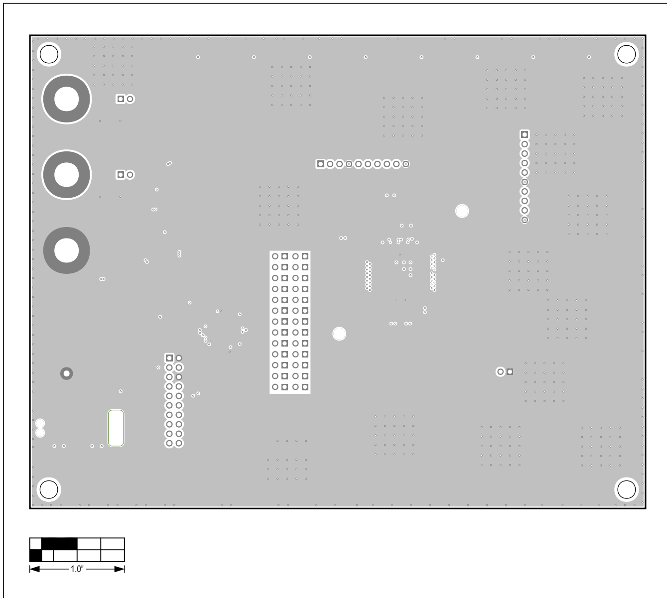
MAX9972 EV Kit PCB Layout—Internal 2 (Ground)
