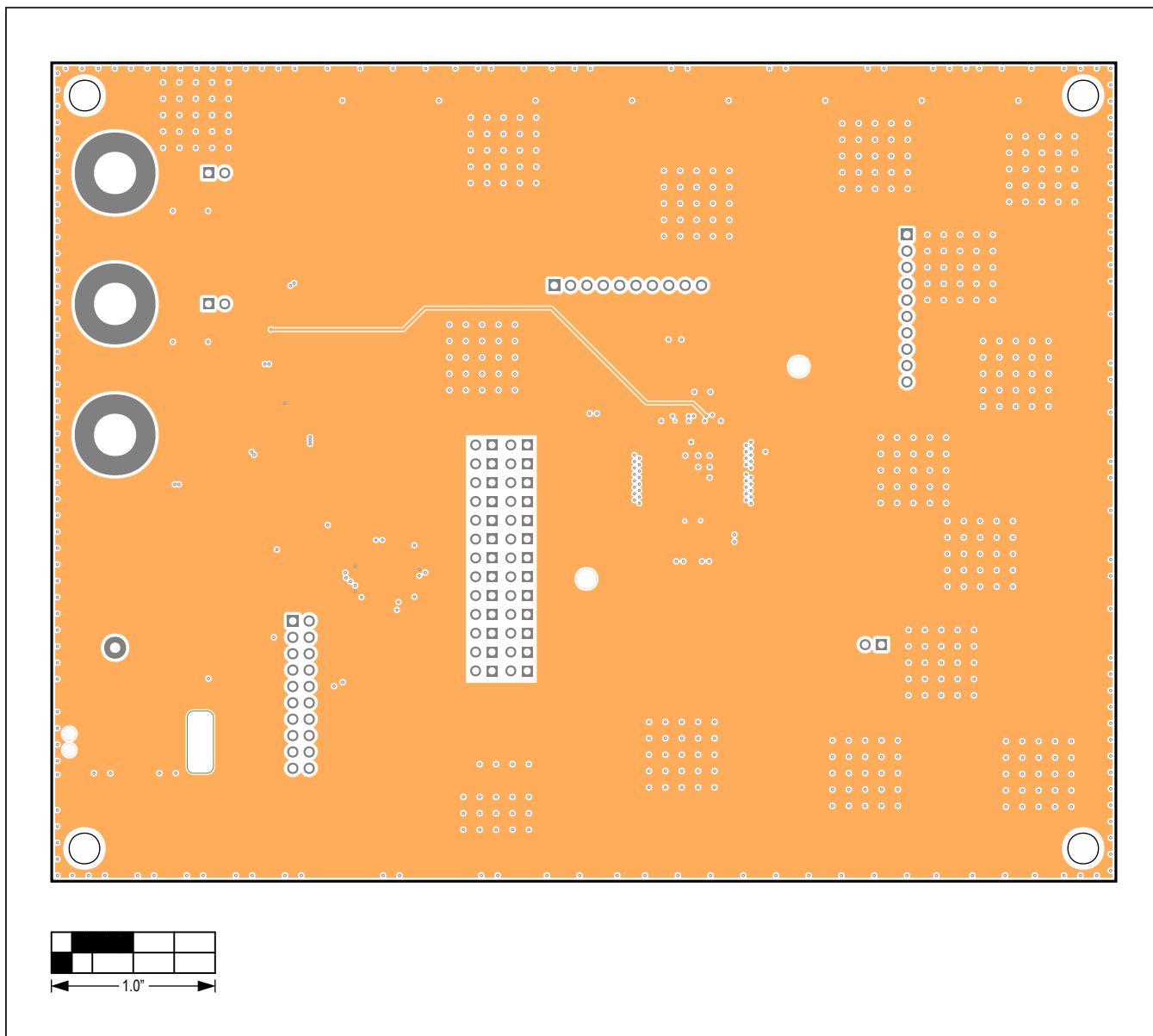
MAX9972 EV Kit PCB Layout—Internal 5 (VDD)
