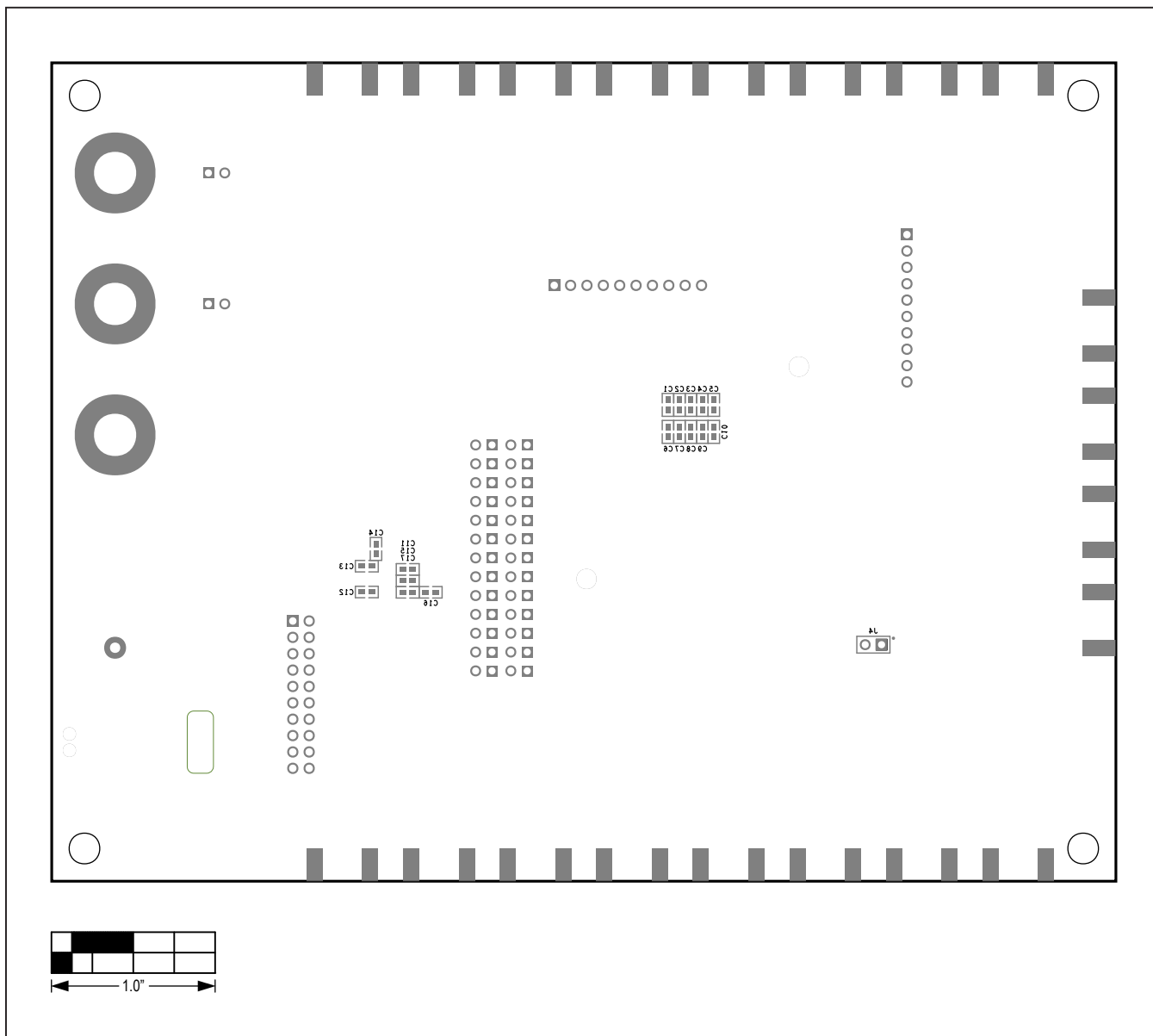
MAX9972 EV Kit PCB Layout—Silkscreen Bottom
