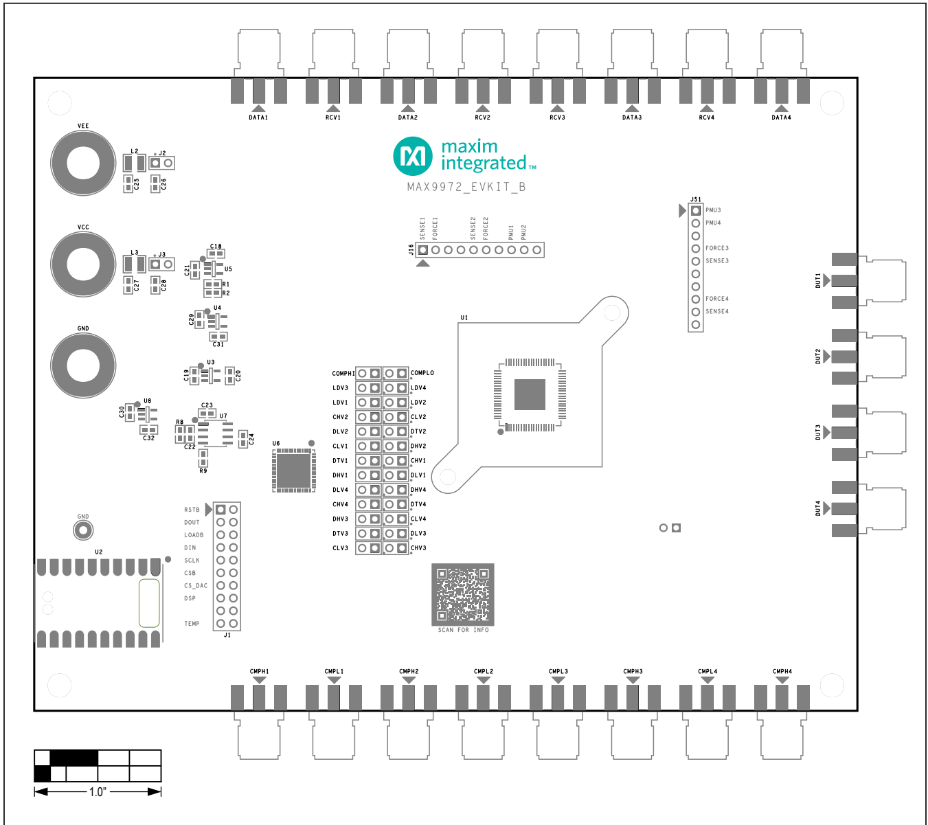
MAX9972 EV Kit PCB Layout—Top Silkscreen
