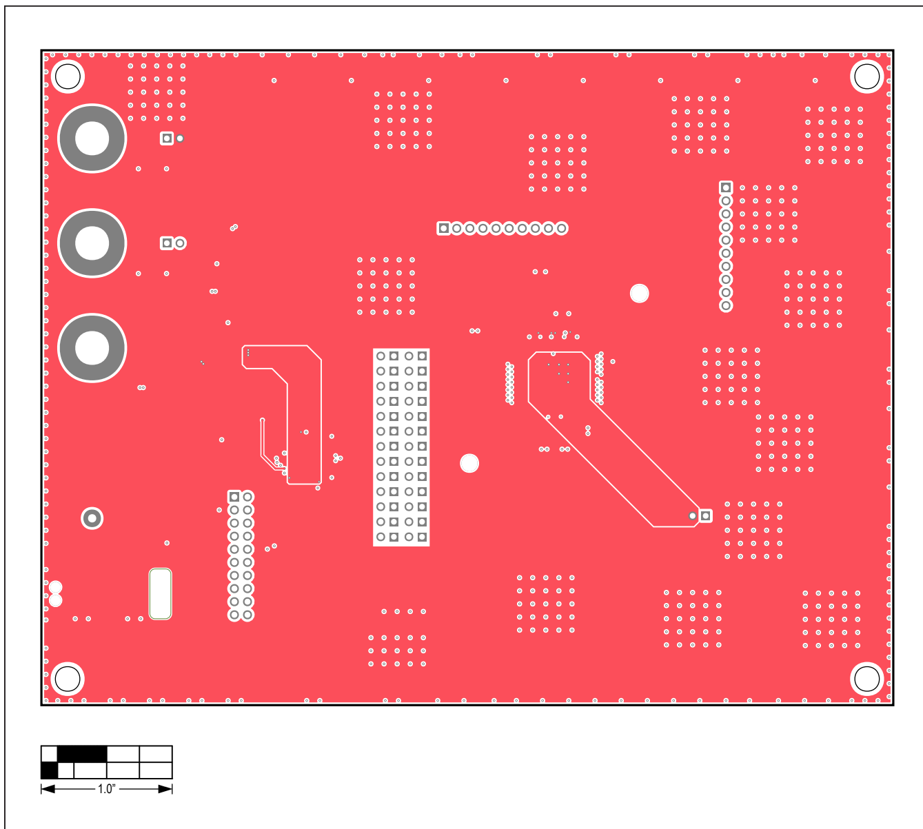
MAX9972 EV Kit PCB Layout—Internal 4 (VEE)
