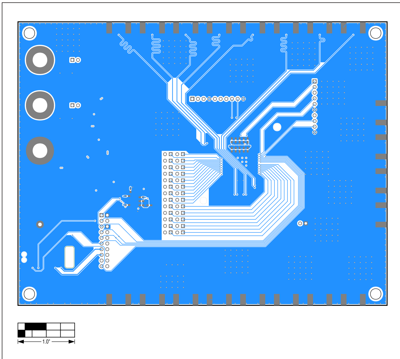
MAX9972 EV Kit PCB Layout—Bottom View
