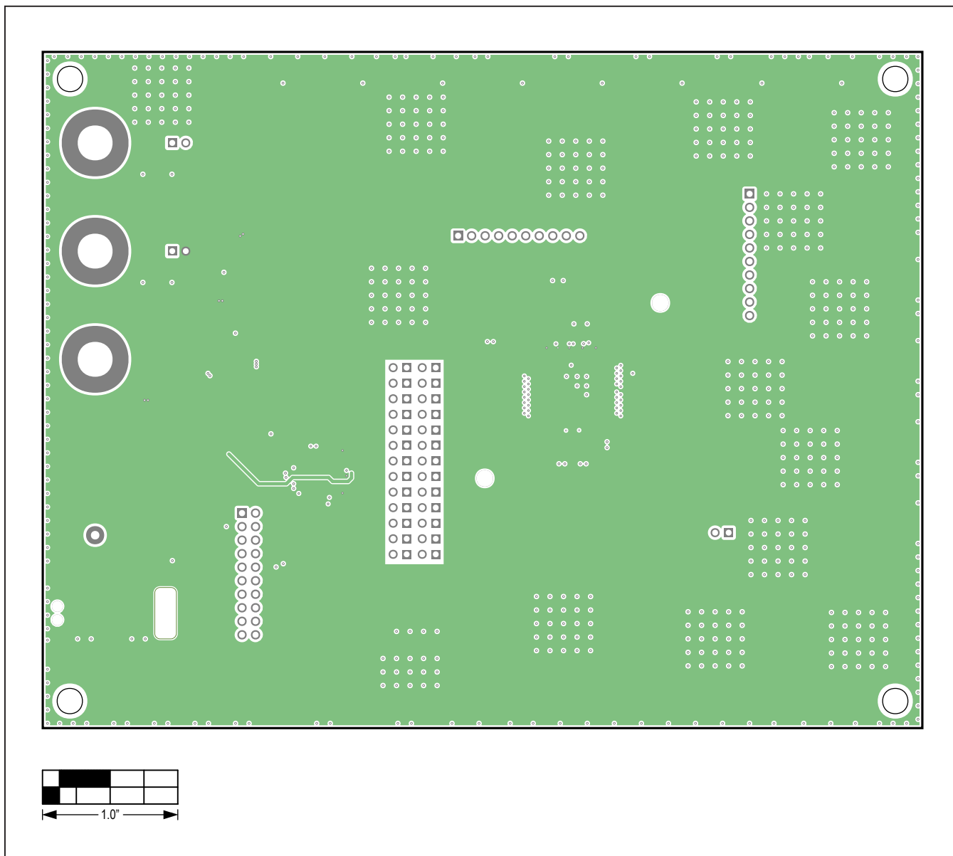
MAX9972 EV Kit PCB Layout—Internal 3 (VCC)
