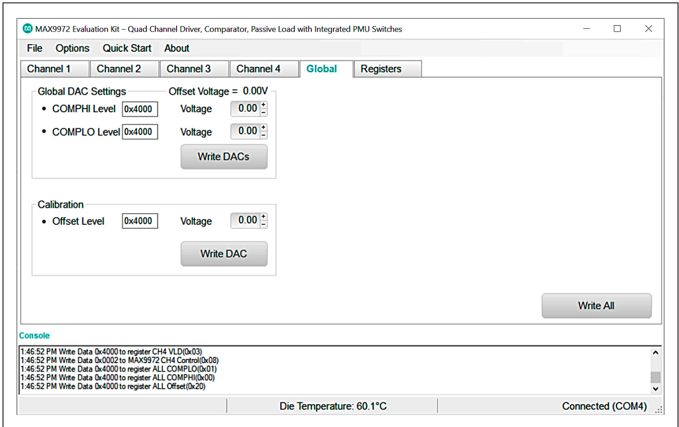
Figure 3. MAX9972 EV Kit Software Window (Level-Setting Channel DACs)
