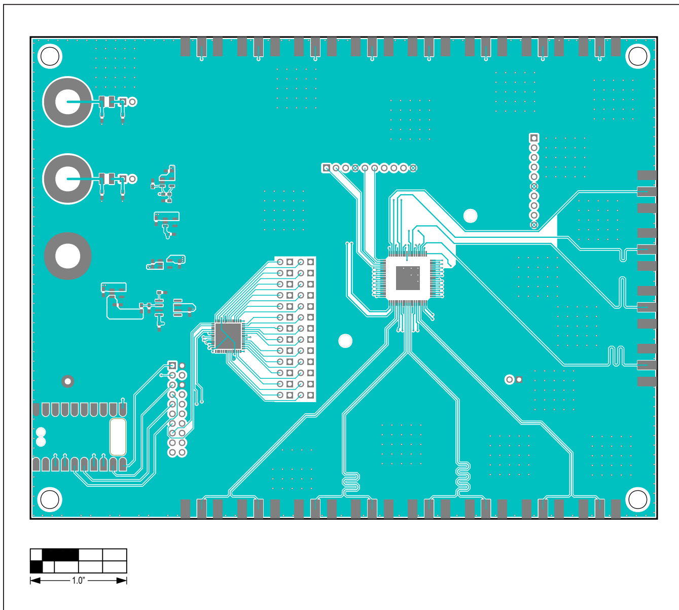
MAX9972 EV Kit PCB Layout—Top View
