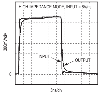
COMPARATOR RESPONSE TO HIGH SLEW-RATE INPUT
