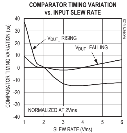
COMPARATOR RESPONSE TO HIGH SLEW-RATE INPUT
