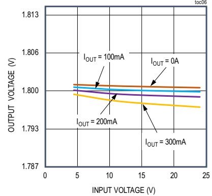
OUTPUT VOLTAGE vs. INPUT VOLTAGE V_{OUT} = 1.8V , PWM MODE
