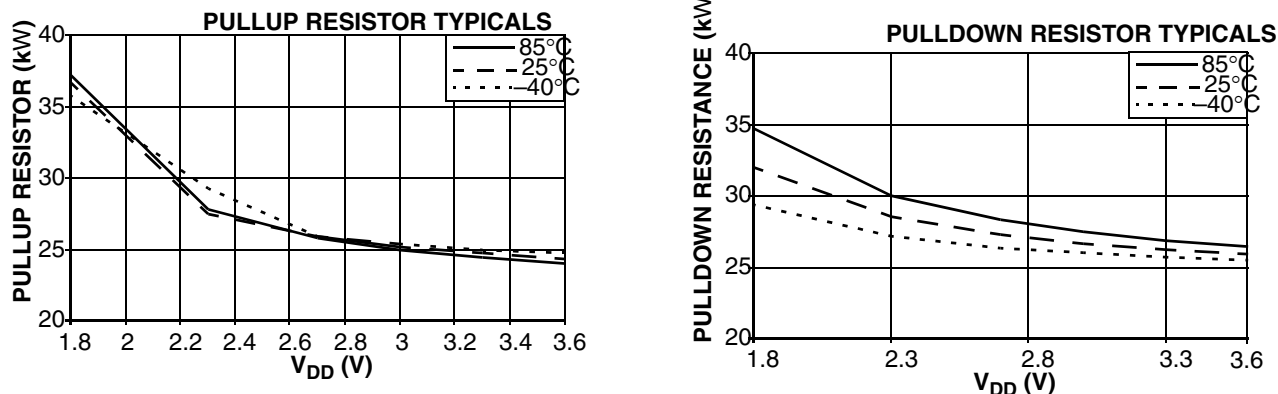
Figure 16. Pullup and Pulldown Typical Resistor Values
