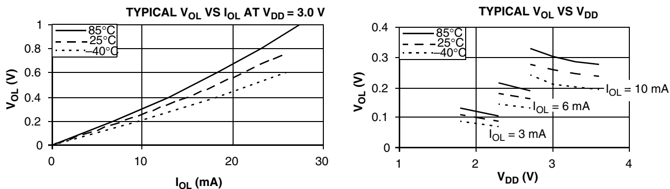
Figure 18. Typical Low-Side Driver (Sink) Characteristics — High Drive (GPIO_x_DRIVEN = 1)
