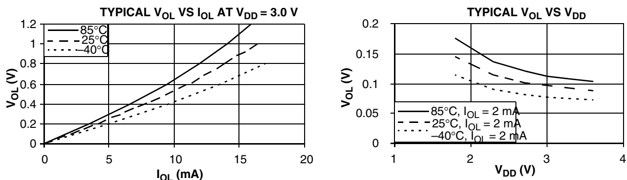
Figure 17. Typical Low-Side Driver (Sink) Characteristics — Low Drive (GPIO_x_DRIVEN = 0)
