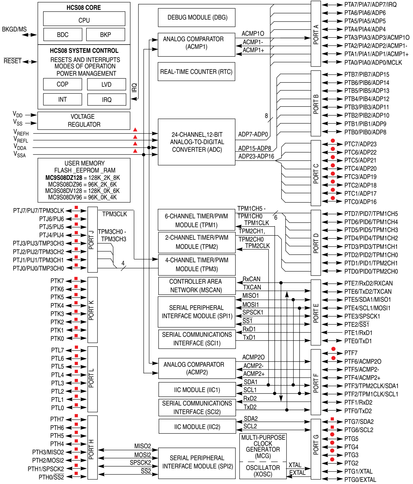
Figure 1-1. MC9S08DZ128 Block Diagram
