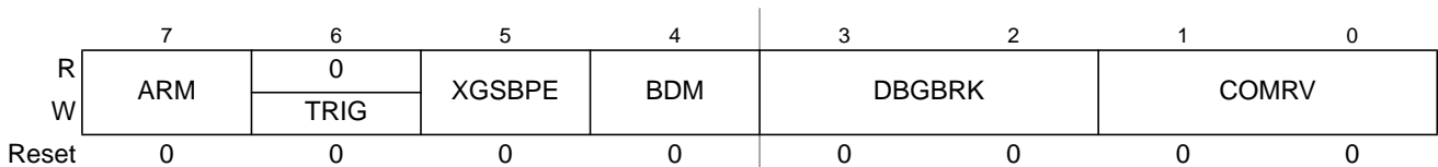
Figure 20-3. Debug Control Register (DBG1)
