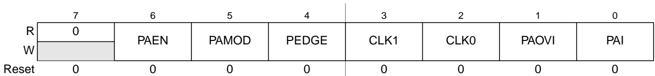
Figure 7-35. 16-Bit Pulse Accumulator Control Register (PACTL)
