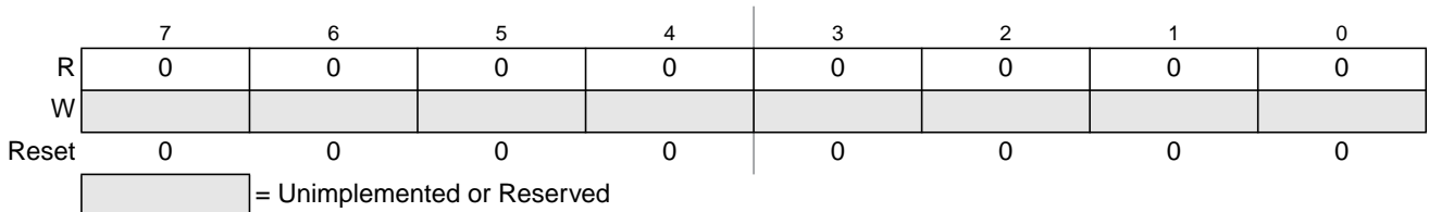
Figure 8-13. Reserved Registers (PWMSCNTx)
