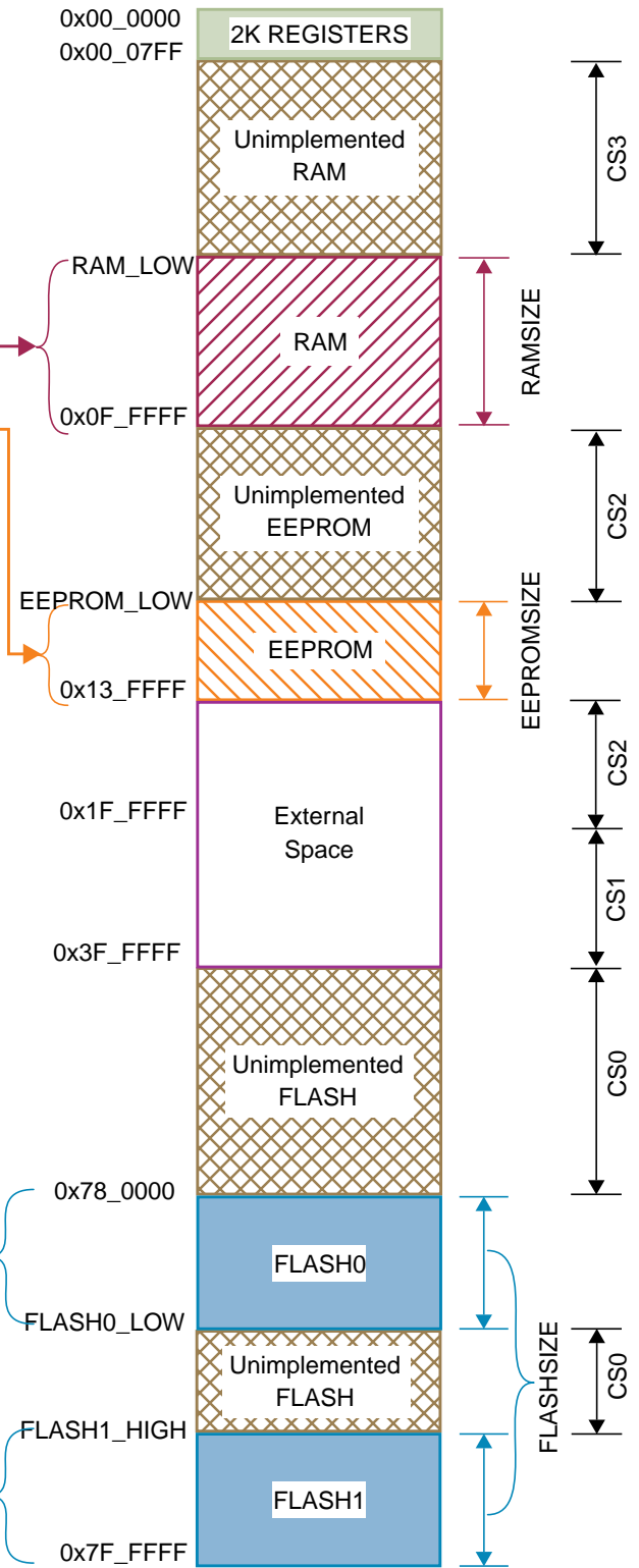
Figure 1-4. S12X CPU & BDM Global Address Mapping
