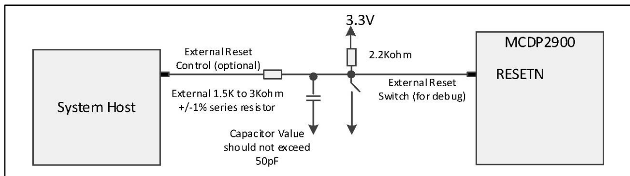
Figure 8. EXT_RESETN Connection to MCDP2900
