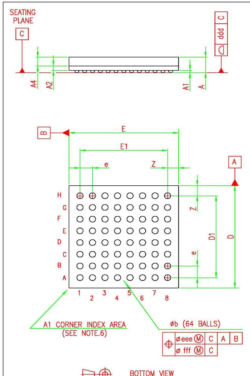
Figure 9. MCDP2900 package drawing
