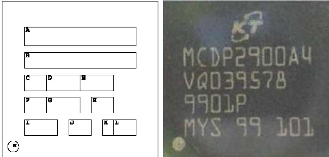
Figure 10. Marking template
