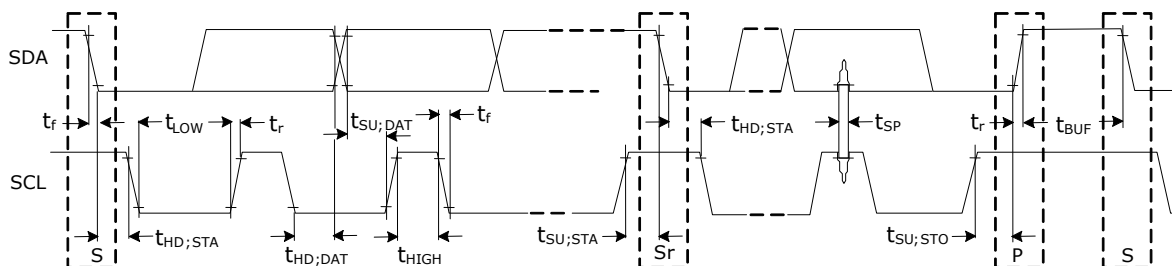
Figure 4. I2C Timing
