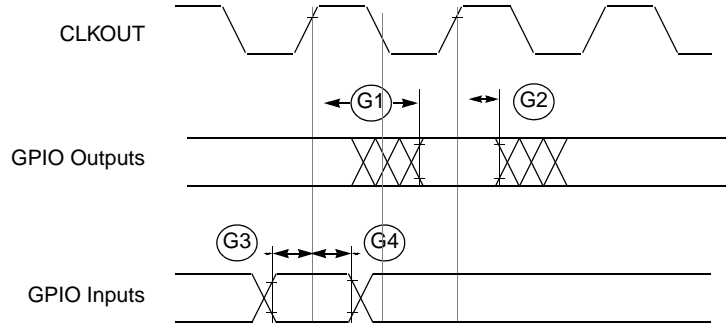
Figure 16. GPIO Timing
