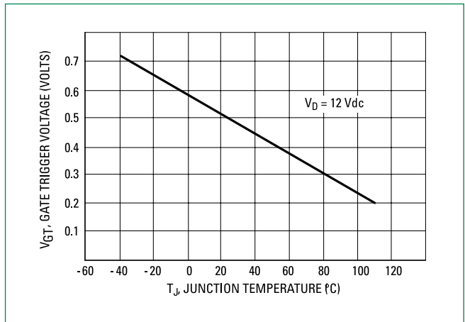
Figure 4. Gate Voltage
