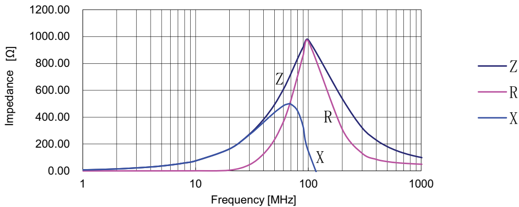
MFBM1V2012-102-R
