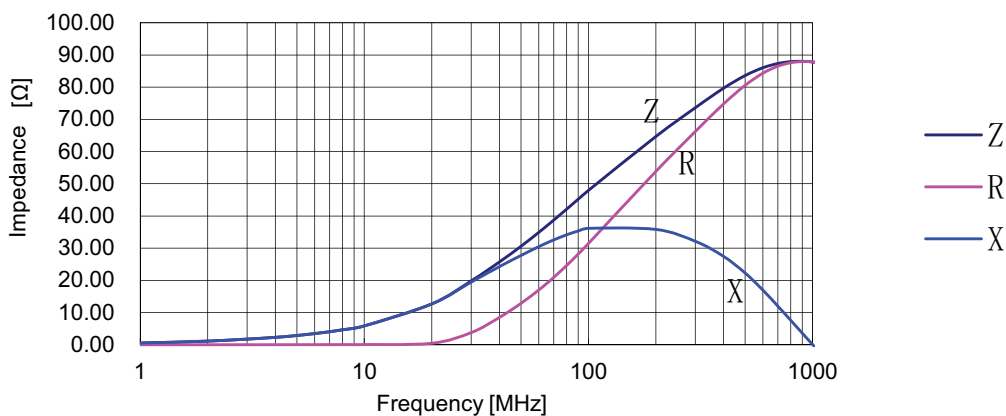
MFBM1V2012-600-R
