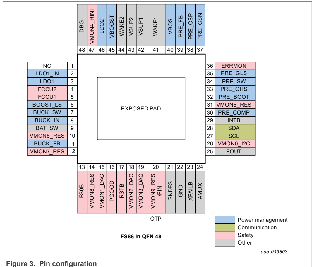
Figure 3. Pin configuration
