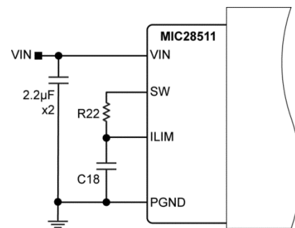
Figure 1. MIC28511 Current Limiting Circuit
