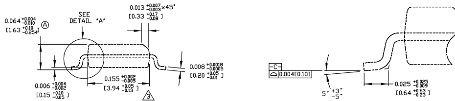
END VIEW
