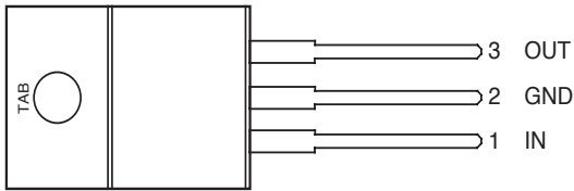
MIC39500-x.xBT TO-220-3 (T)
