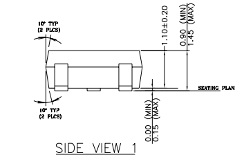
SIDE VIEW 1
