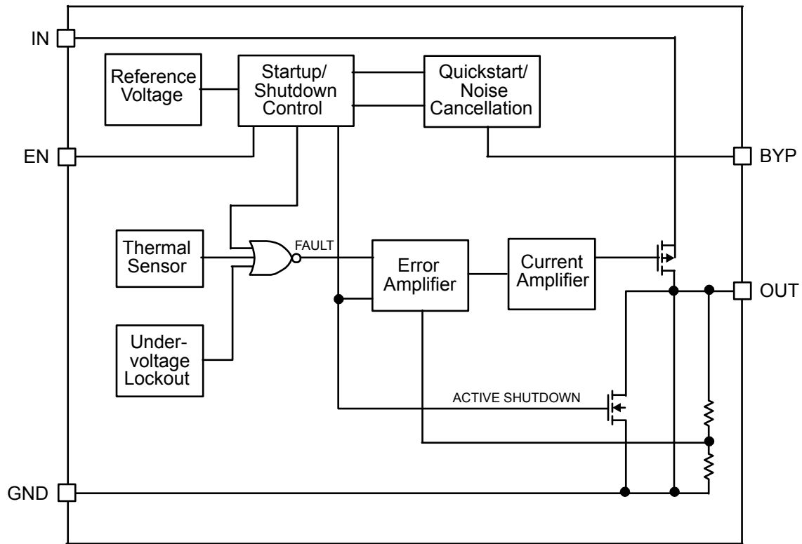
MIC5265 Diagram
