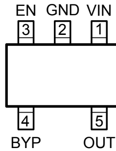
Lead-Free Thin SOT-23-5 (M5)
