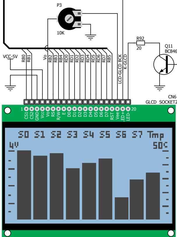
Figure 12-1: GLCD 128x64 connection schematic
