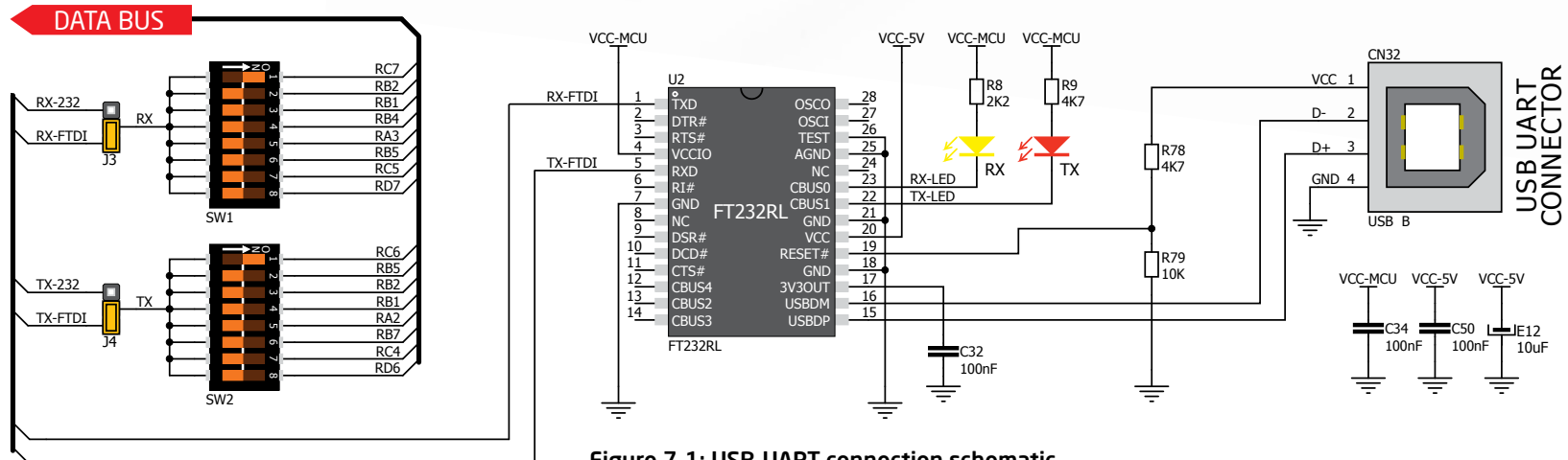
Figure 7-1: USB-UART connection schematic
