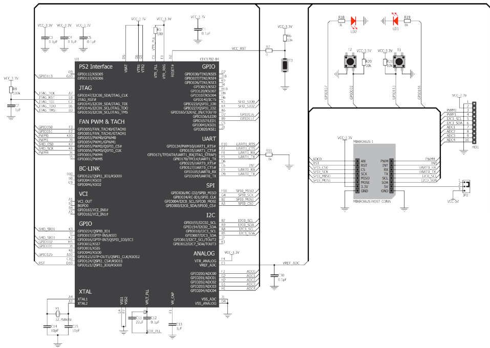
Figure 5-2: Other modules connection schematic
