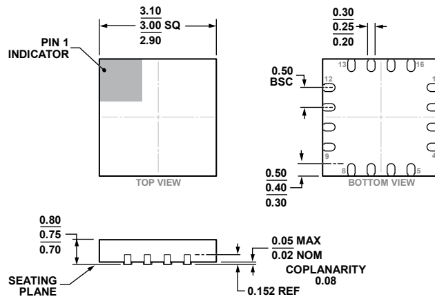
Figure 43. 16-Lead Lead Frame Chip Scale Package [LFCSOP] 3 mm x 3 mm Body and 0.75 mm Package Height (CP-16-32)
