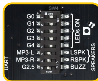
Figure 19: SW4.1 through SW4.5 switches are used to enable group LEDs
