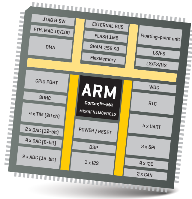
Figure 1: MK66FX1M0VLQ18 MCU block schematic
