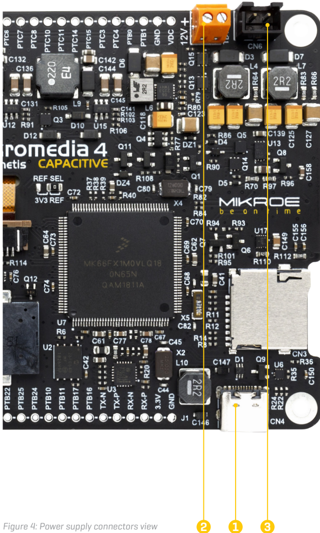
Figure 4: Power supply connectors view
