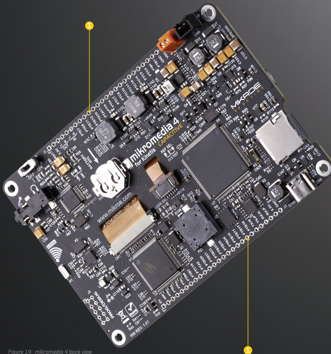
Figure 14: mikromedia 4 back view
