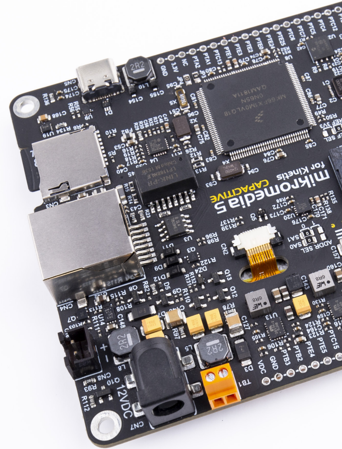
Figure 15: mikromedia 5 back view
