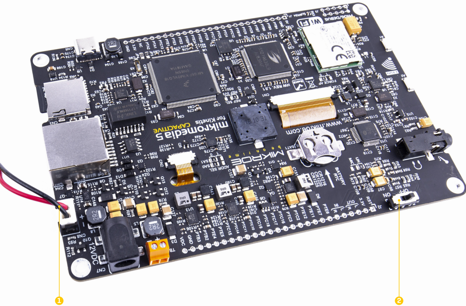
Figure 8: Battery power supply connection
