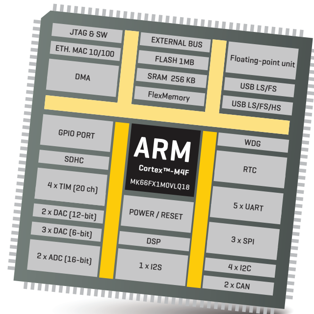
Figure 1: Kinetis MK66FX1MOVQ18 MCU block schematic
