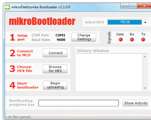
Figure 2-1: mikroBootloader window
