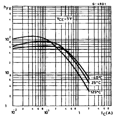
Figure 4. DC current gain ( V_{CE} = 5V )
