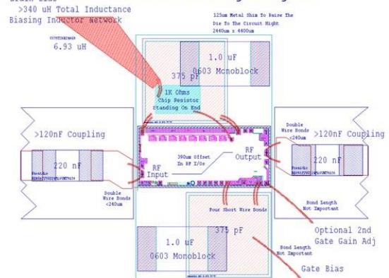
30KHz - 30GHz bonding diagram
