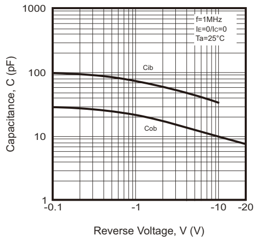
Fig.5 - C_{ob}/C_{ib} — V_{CB}/V_{EB}
