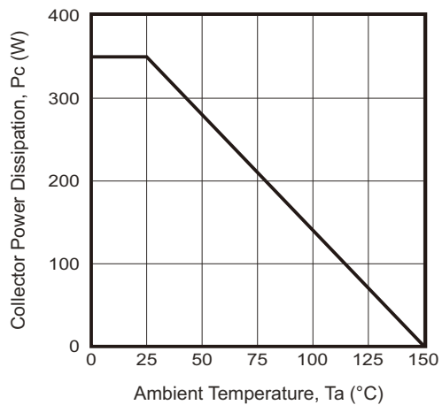
Fig.7 - P_C — T_a
