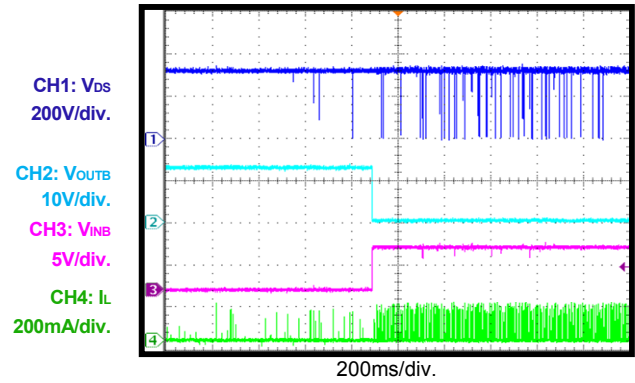
Relay 2 Turn-On No Load
