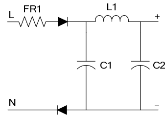
Figure 6: Half-Wave Rectifier
