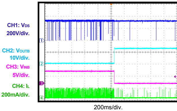
Relay 2 Turn-Off No Load
