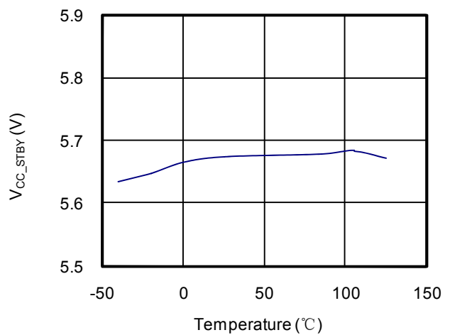
V_{CCSTBY} vs. Temperature
