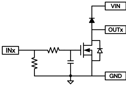
Figure 4: Block Diagram of Internal Relay Driver
