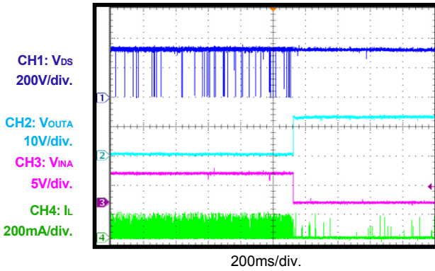
Relay 1 Turn-Off No Load
