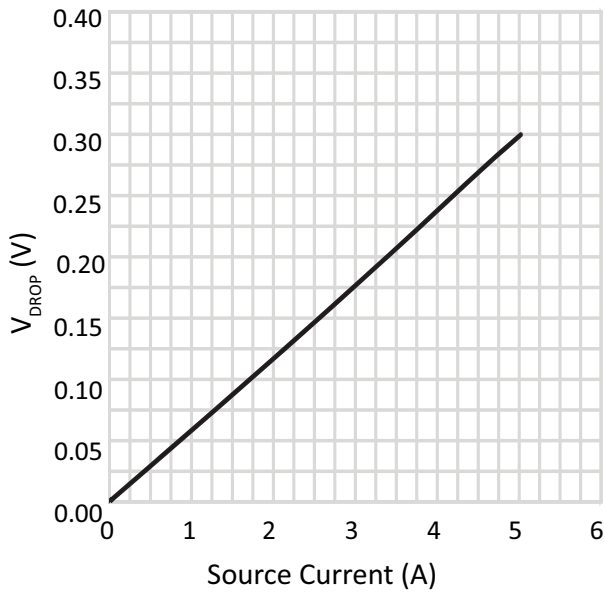
Figure 9: Typical Source Voltage Drop +V B = +V S + 6V
