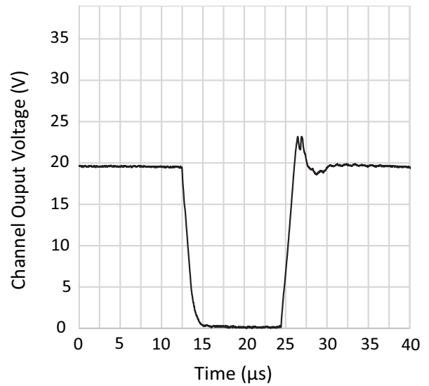
Figure 14: Single Pulse Output Voltage C_{LOAD} = 320\text{nF}
