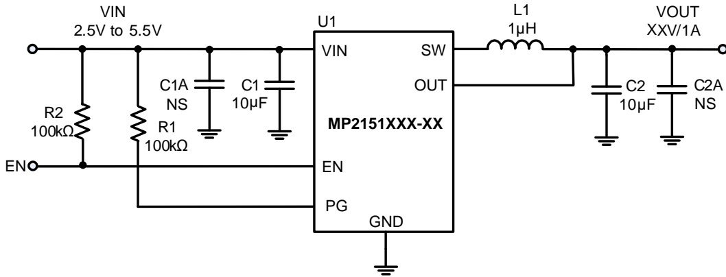
Figure 12: Typical Application Circuit for MP2151XXX-XX NOTE: VIN < 3.3V applications may require more input capacitors.
