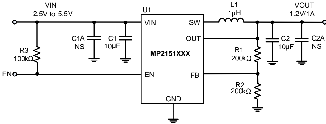
Figure 11: Typical Application Circuit for MP2151XXX NOTE: VIN < 3.3V applications may require more input capacitors.
