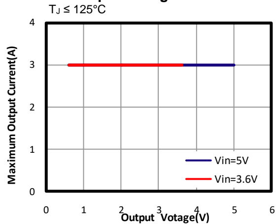
Output Current Derating vs. Output Voltage T J ≤ 125°C
