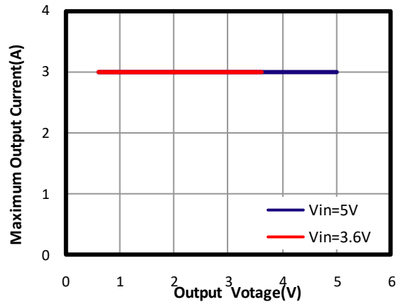
Output Current Derating vs. Output Voltage T J ≤ 125 ^{\circ} C
