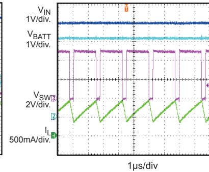
CV Charge Steady State
