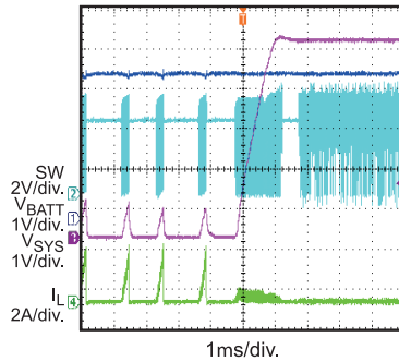
SYS Short Circuit Recovery
