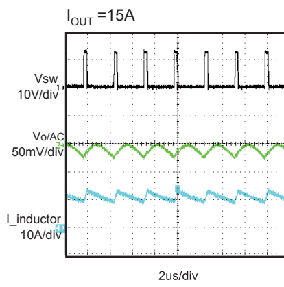
Output Ripple
