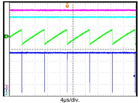
Low-Dropout Mode
