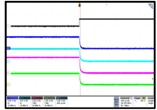
CH1/CH2 Shutdown through EN
