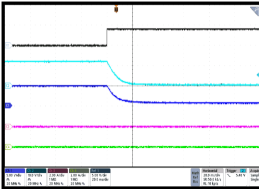
CH1/CH2 Shutdown through EN
