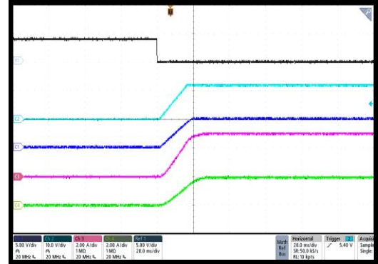
CH1/CH2 Start-Up through EN
