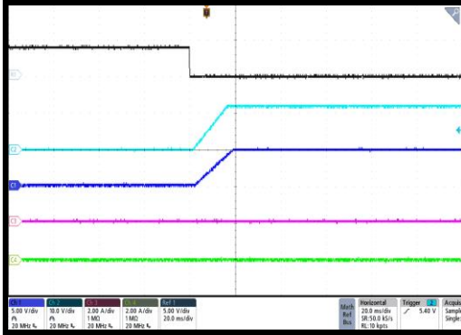
CH1/CH2 Start-Up through EN
