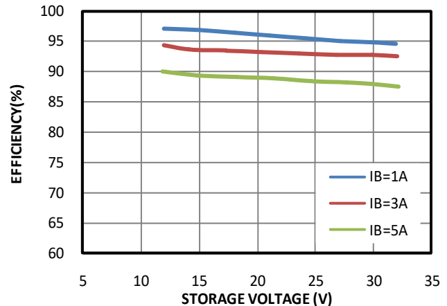
Buck Efficiency
