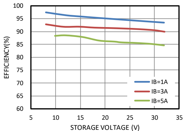
Buck Efficiency
