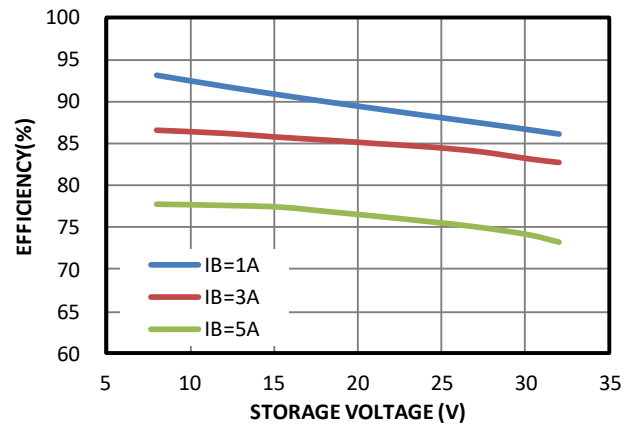
Buck Efficiency
