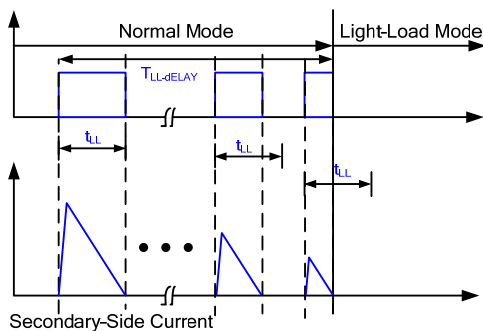
Figure 5: MP6906 Enters Light-Load Mode
