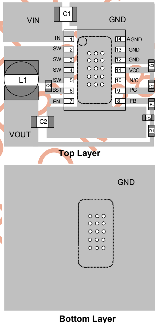
Figure 7—PCB Layout
