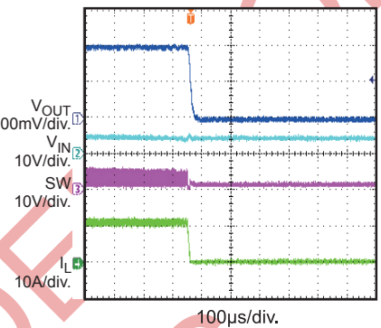
Shutdown Through V_{IN} I_{OUT} = 12A
