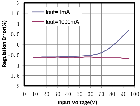
Line Regulation
