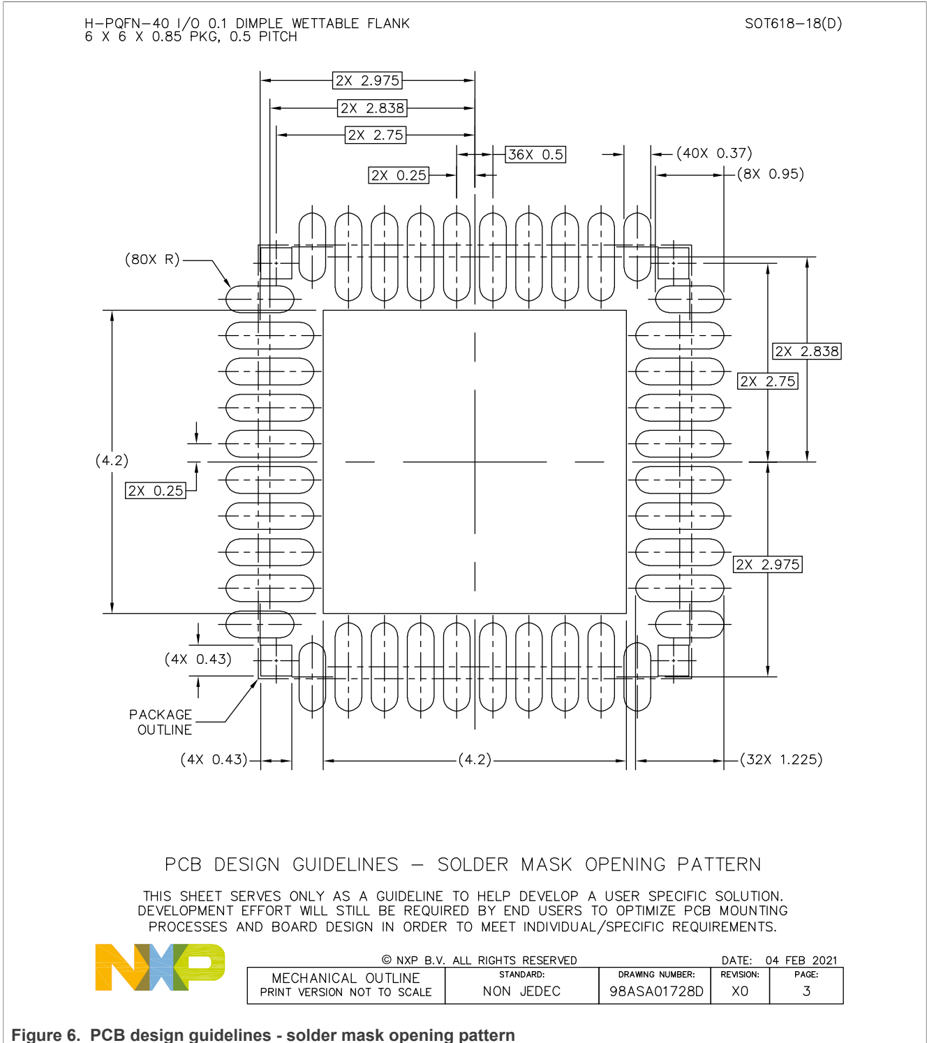
Figure 6. PCB design guidelines - solder mask opening pattern
