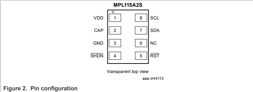
Figure 2. Pin configuration
