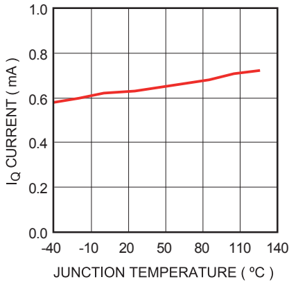
I_Q Current vs. T_J
