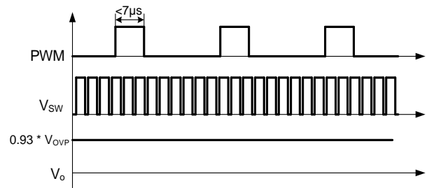
Figure 4: Deep Dimming Ratio for PWM Dimming
