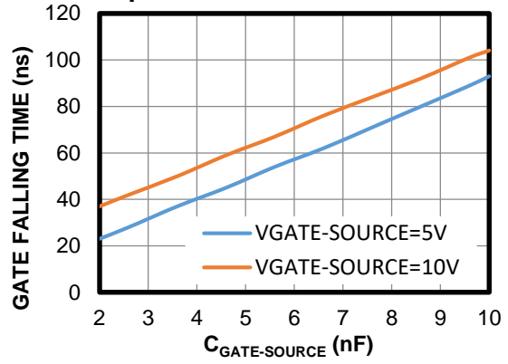
Gate Falling Time vs. Gate Capacitance
