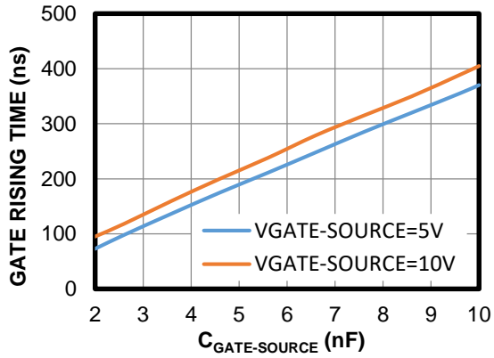
Gate Rising Time vs. Gate Capacitance
